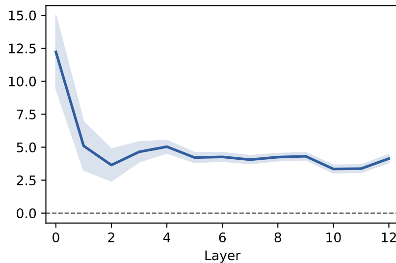
Nonlinear ID
