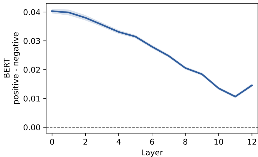
IsoScore
