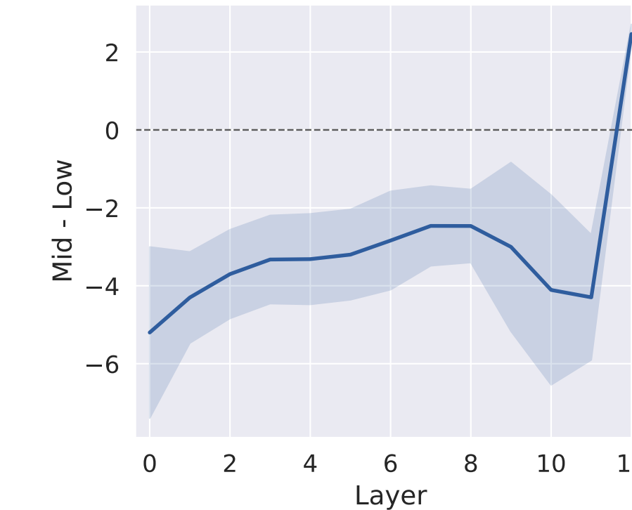
GPT Nonlinear ID
