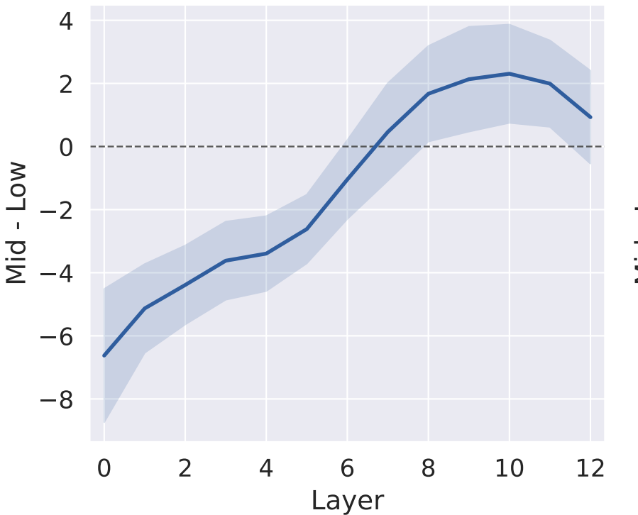
BERT Nonlinear ID
