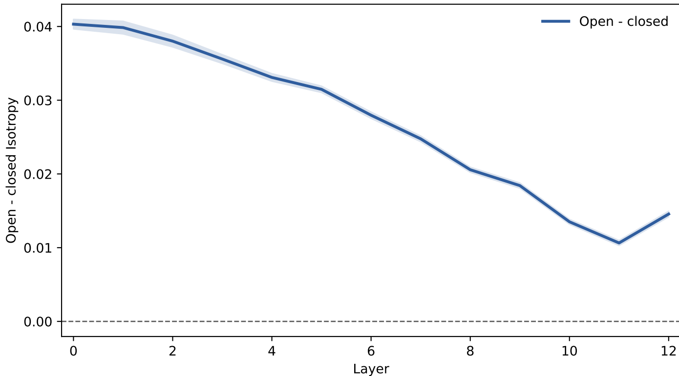
BERT POS open - closed classes (Isotropy)
