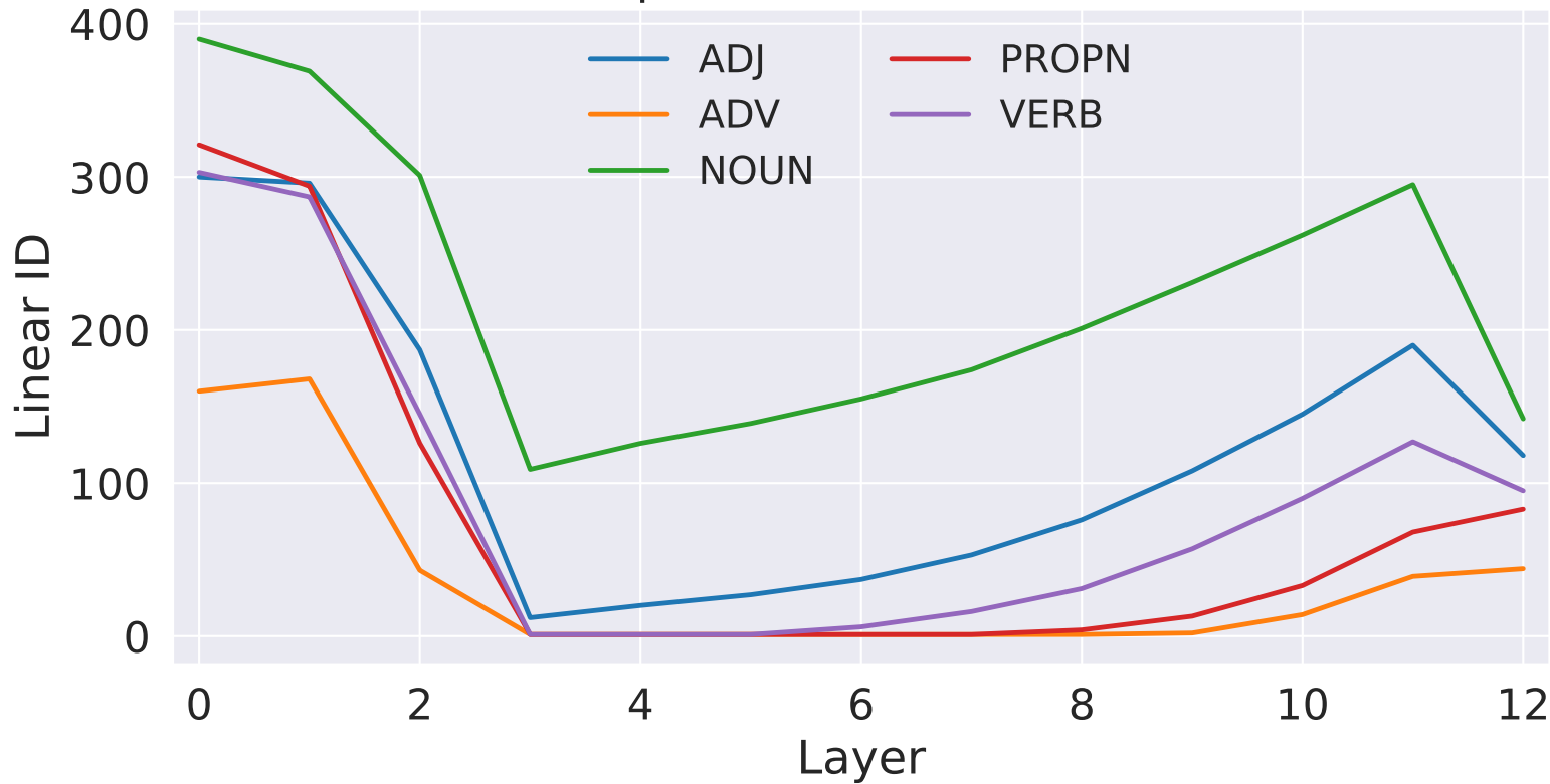
GPT open-class POS (Linear ID)
