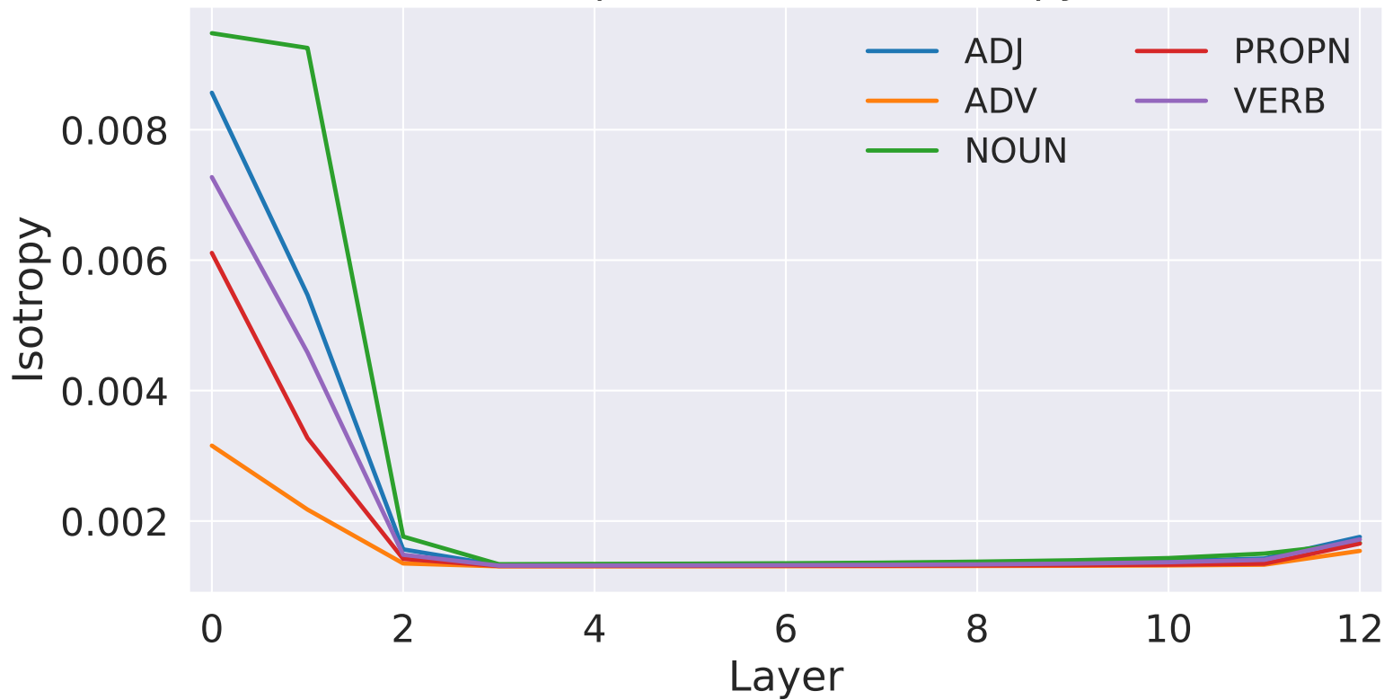
GPT open-class POS (Isotropy)
