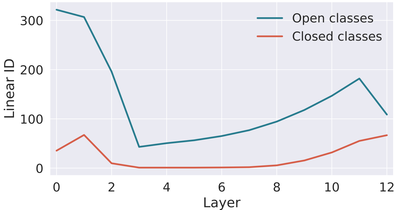
GPT POS open vs closed classes (Linear ID)
