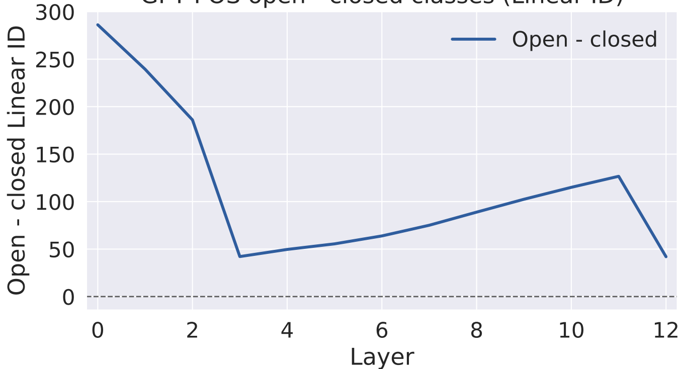
GPT POS open - closed classes (Linear ID)
