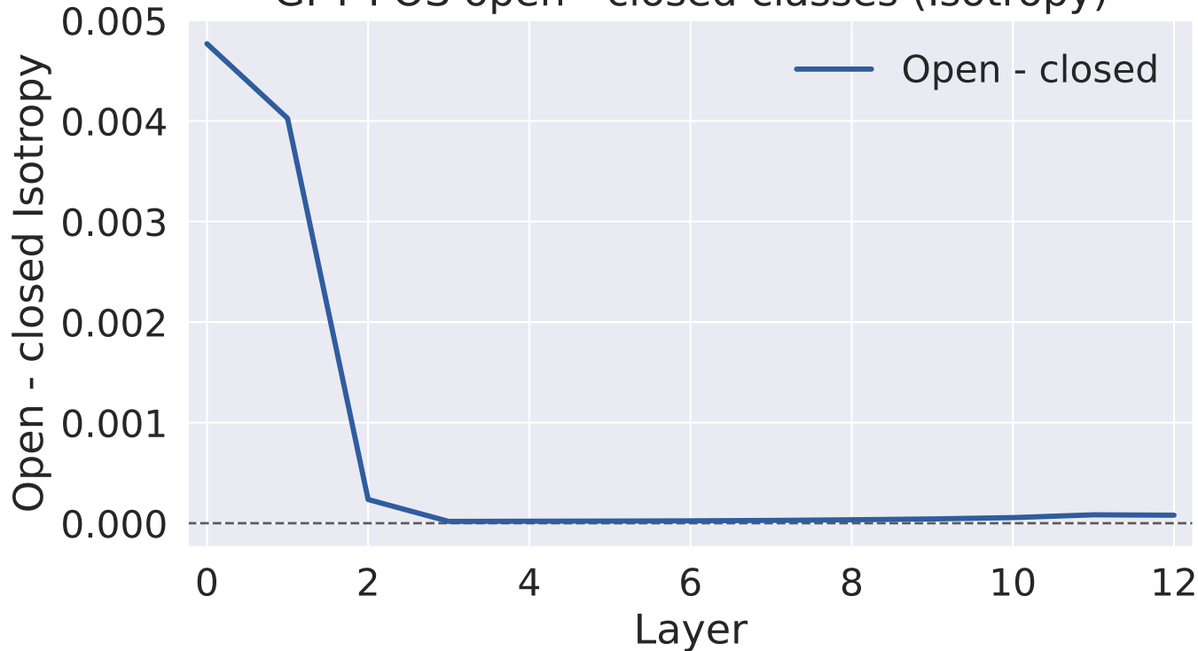
GPT POS open - closed classes (Isotropy)
