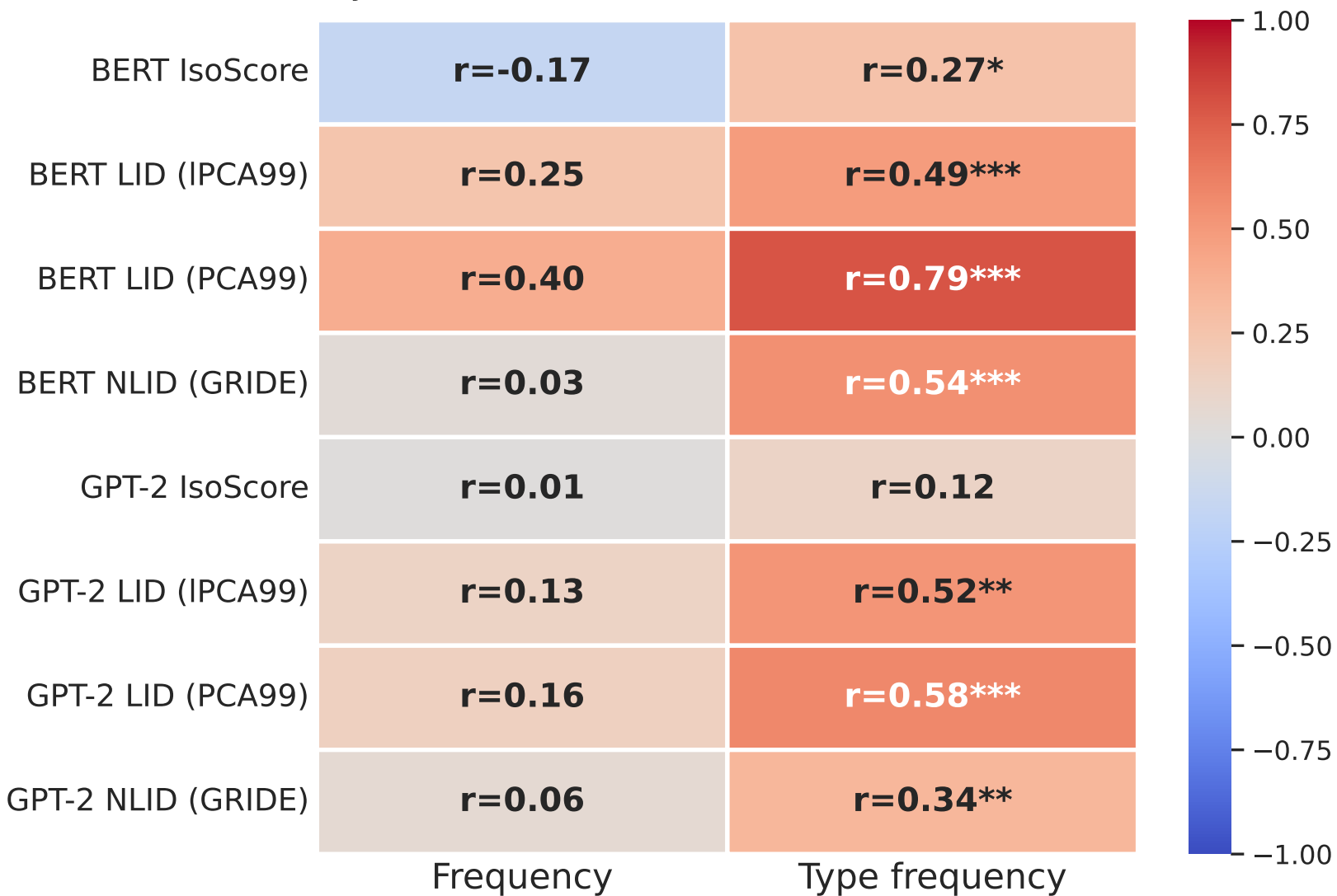
Last-layer uncontrolled metric-count correlations (Pearson)
