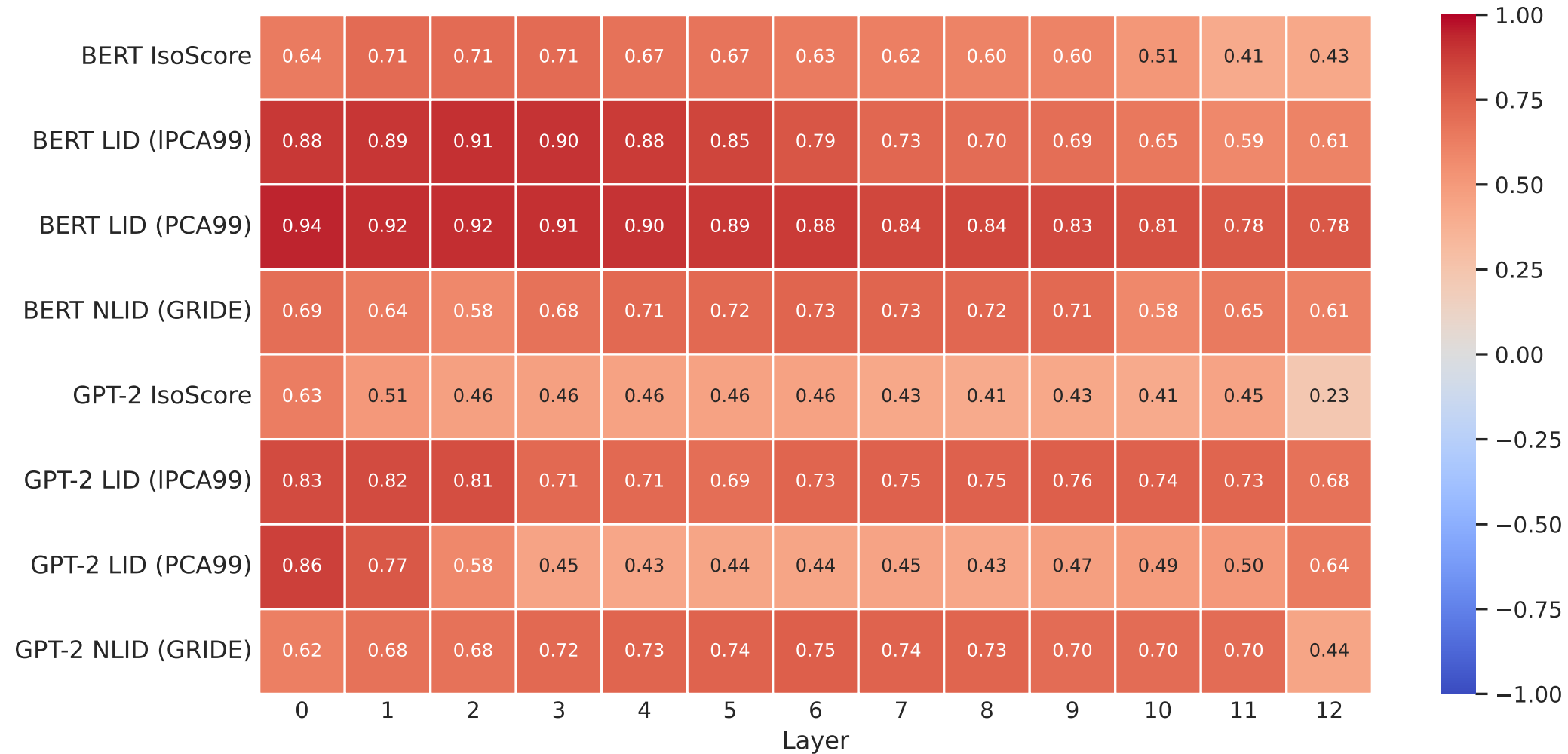
Layerwise uncontrolled Spearman correlations with type frequency
