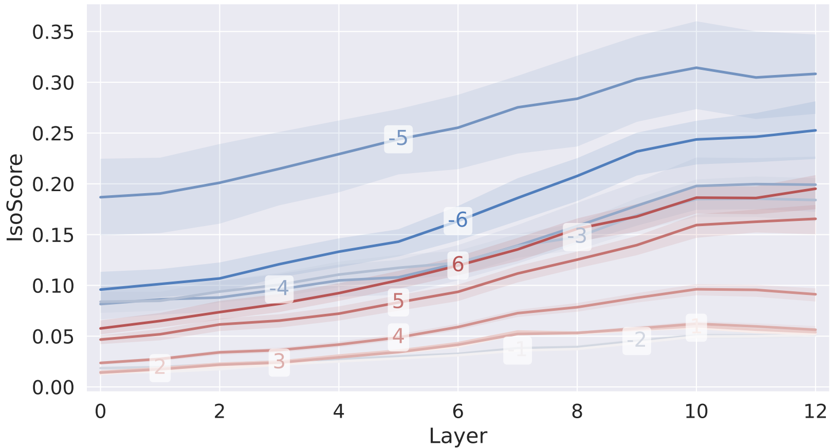
PRON head distance - BERT
