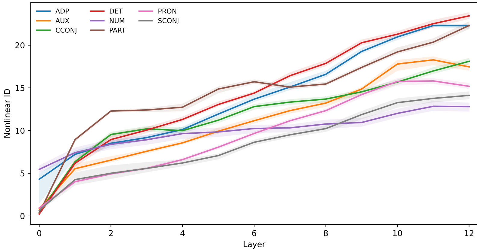
BERT closed-class POS (Nonlinear ID)
