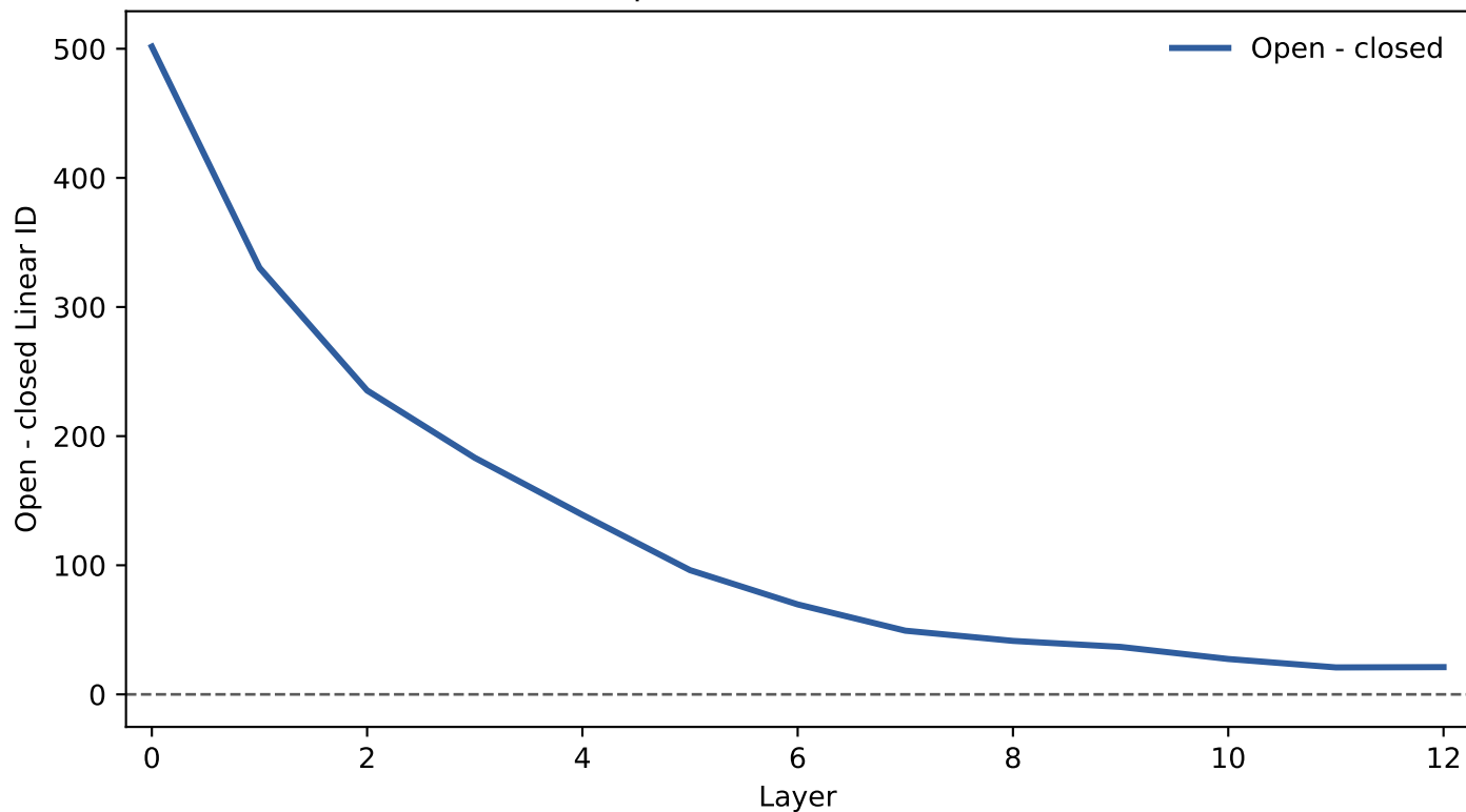
BERT POS open - closed classes (Linear ID)
