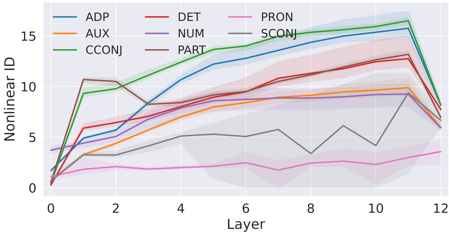
GPT closed-class POS (Nonlinear ID)
