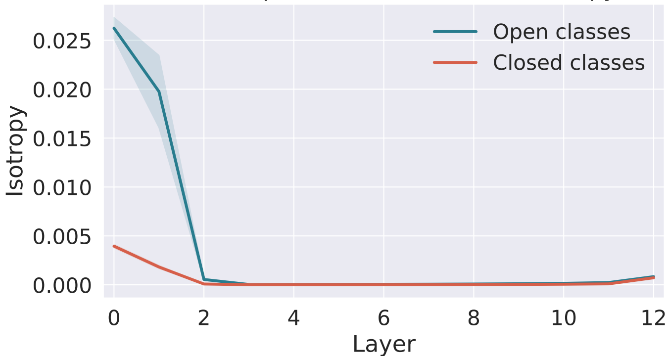
GPT POS open vs closed classes (Isotropy)
