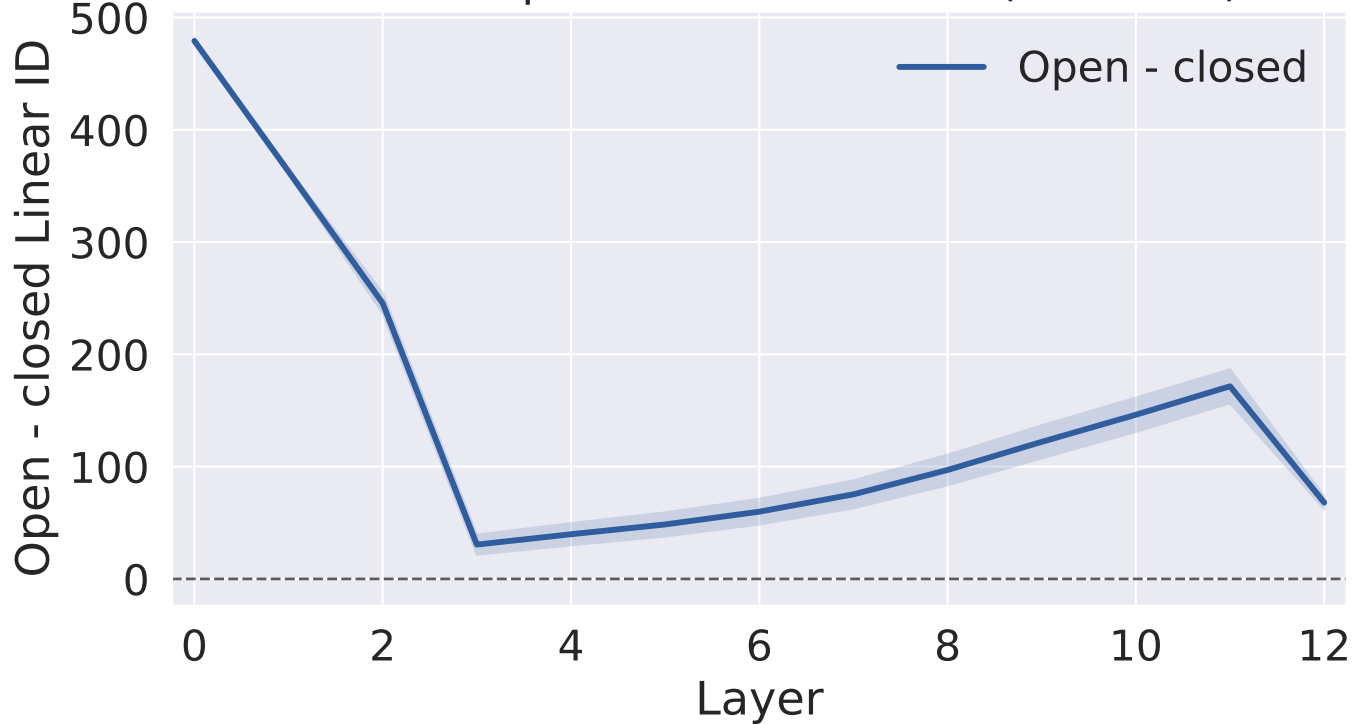
GPT POS open - closed classes (Linear ID)
