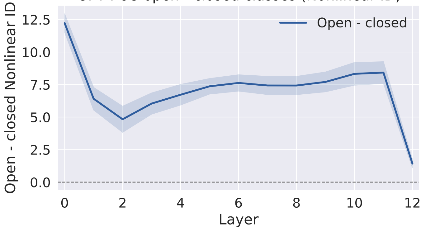
GPT POS open - closed classes (Nonlinear ID)
