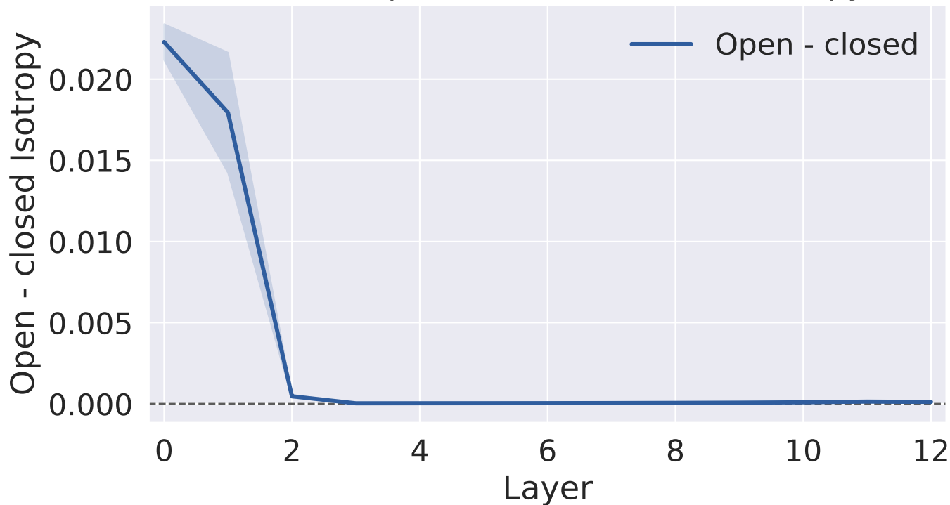
GPT POS open - closed classes (Isotropy)
