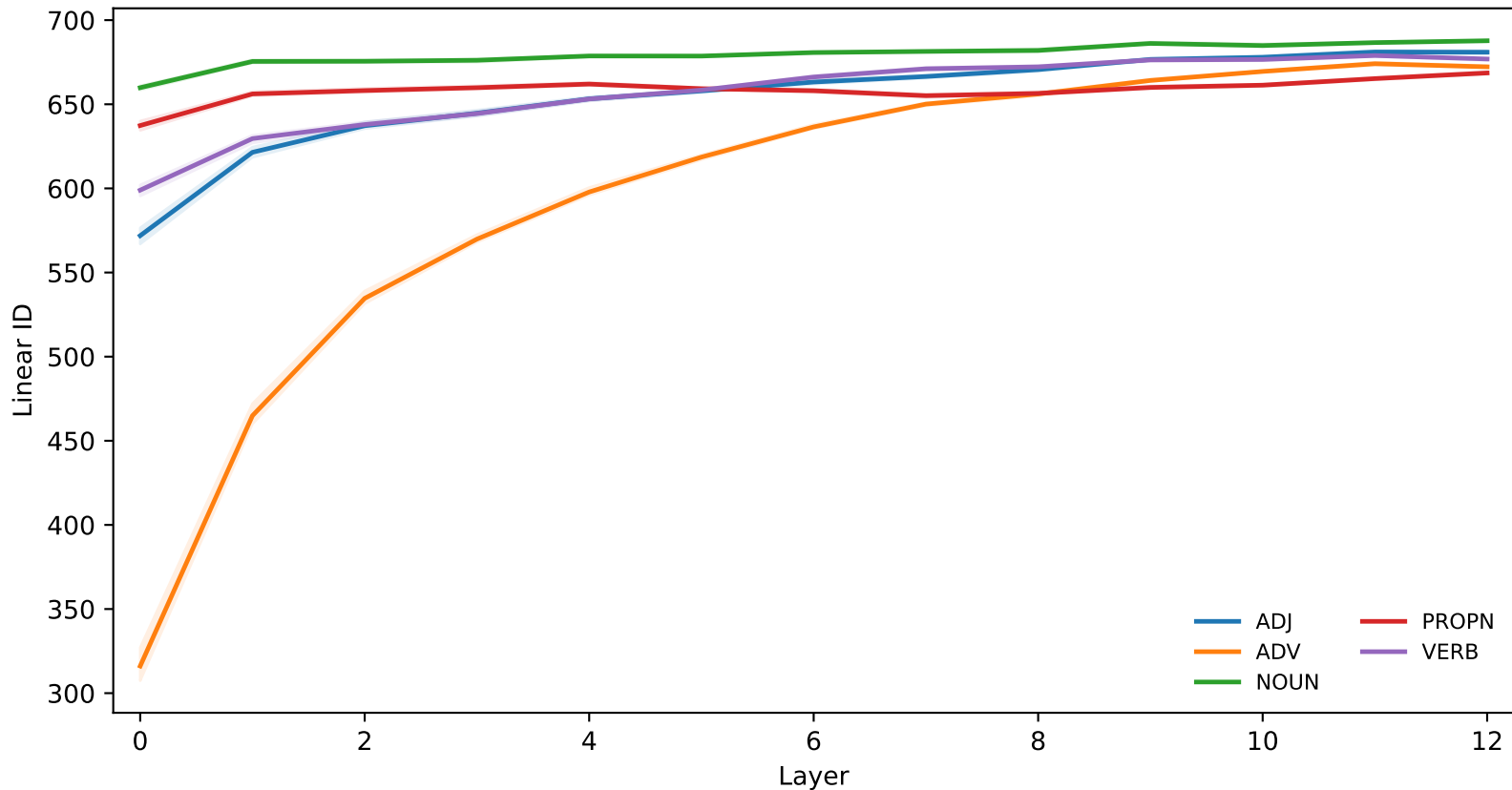
BERT open-class POS (Linear ID)
