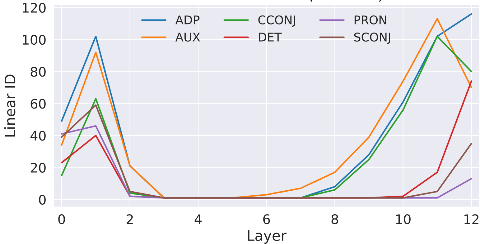
GPT closed-class POS (Linear ID)
