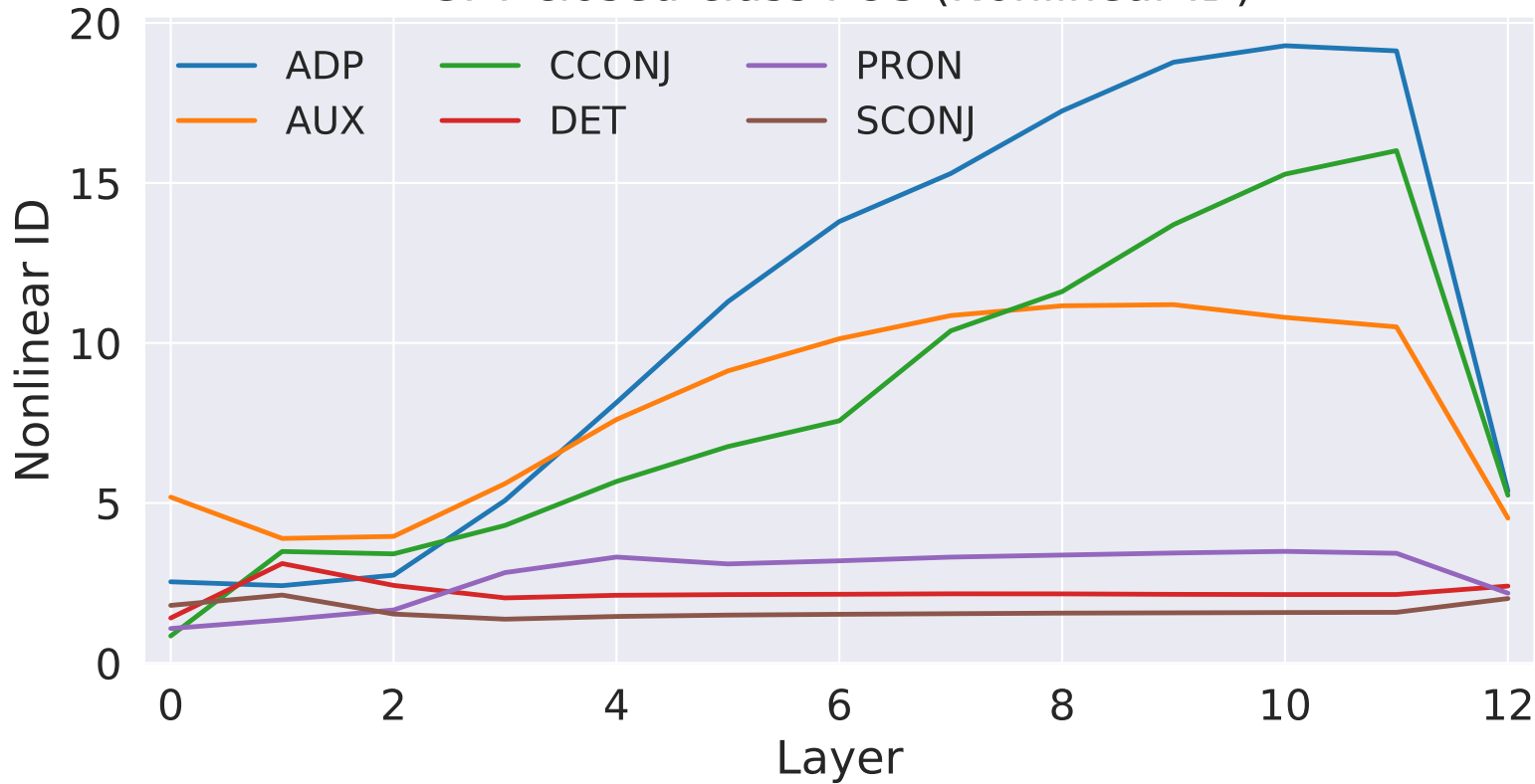
GPT closed-class POS (Nonlinear ID)
