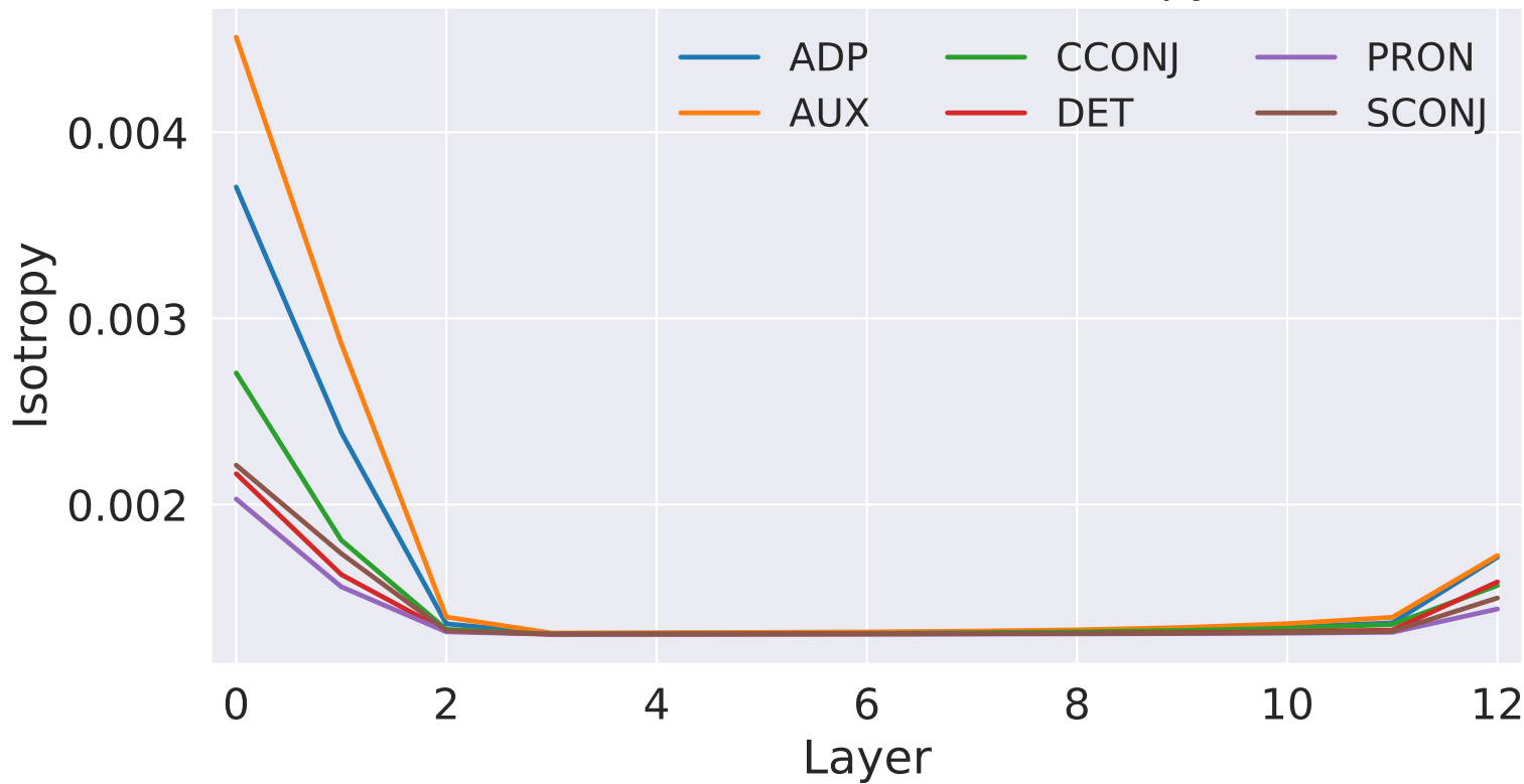
GPT closed-class POS (Isotropy)
