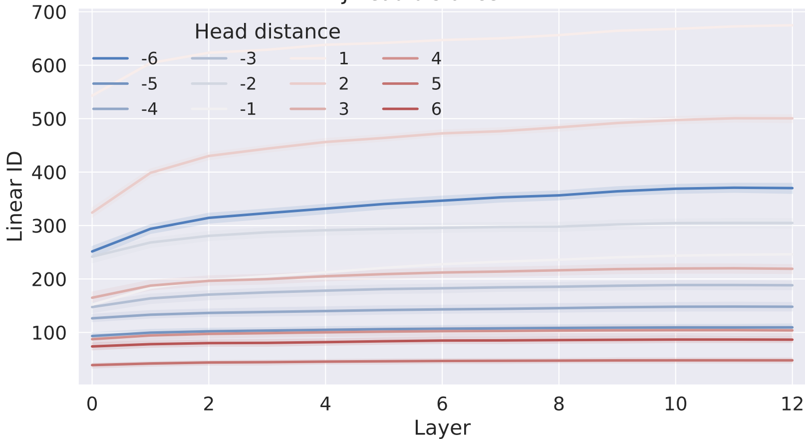
ADJ head distance - BERT
