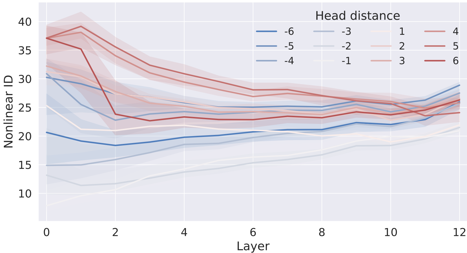
NOUN head distance - BERT
