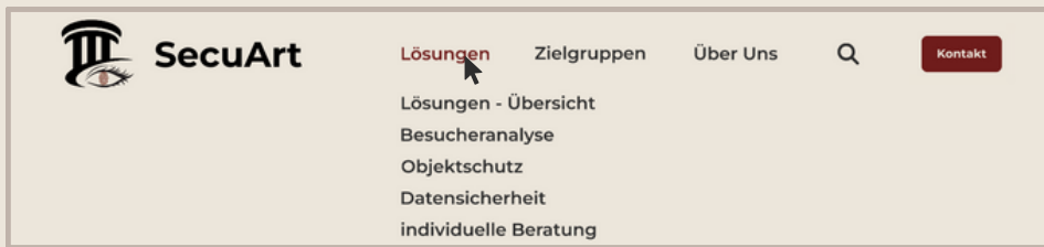
Overlay-Navigation
