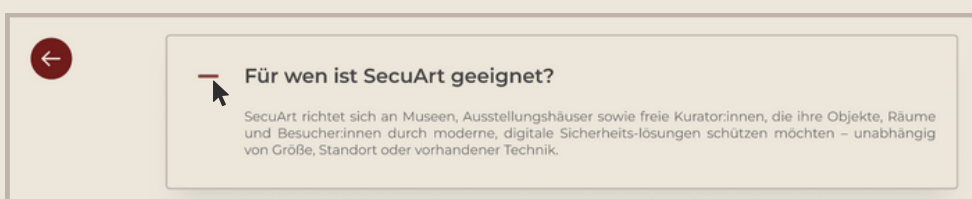
Overlay-FAQ
