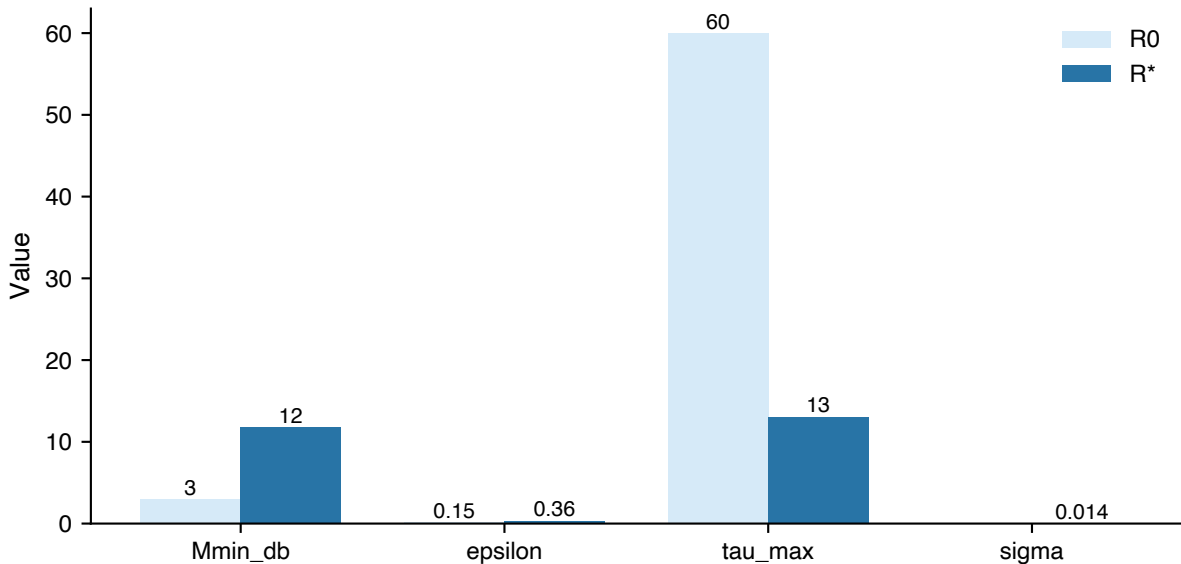
R0 (generic) vs R* (calibrated) thresholds
