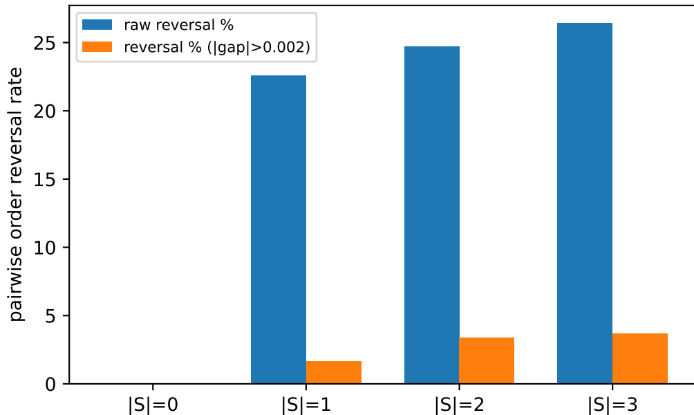
Context rank reversal vs singleton ranking (calib64, U6 base)
