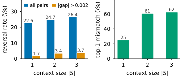
Fig. 1. Singleton-vs-conditional ranking under growing context: (a) pairwise order reversal rate (all pairs vs. large-gap pairs, |gap| > 0.002 ); (b) top-1 mismatch rate.
