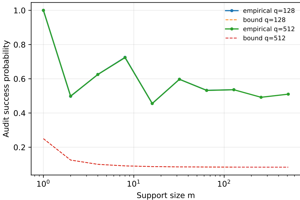
Support-size audit bound (diffuse gradients)
