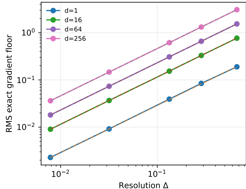
Phase-averaged RMS scaling
