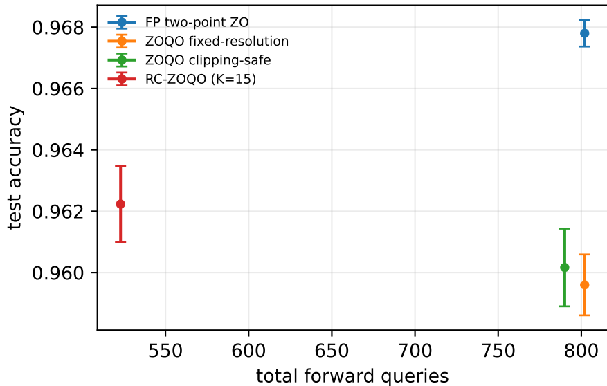
4-bit quantized ZO adaptation
