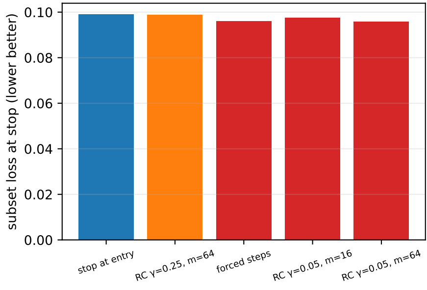
8-bit head-only adaptation
