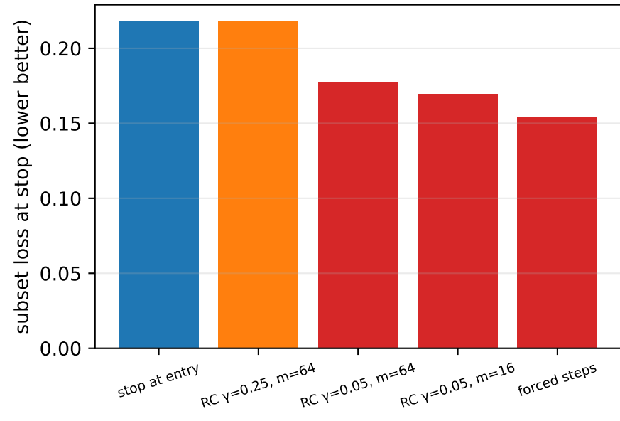
4-bit head-only adaptation
