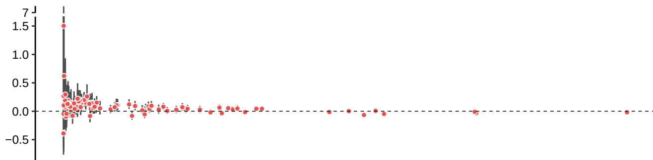
Station data – Extreme high temperature
