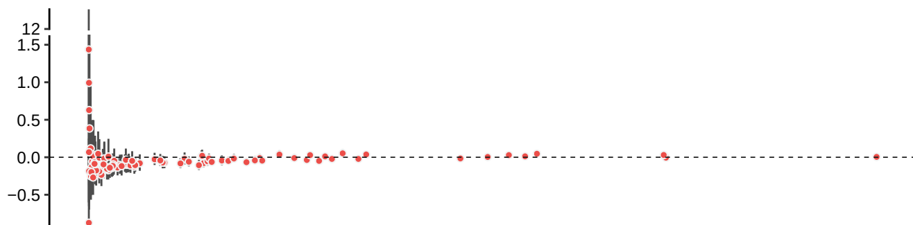
ERA5 data – Extreme high temperature
