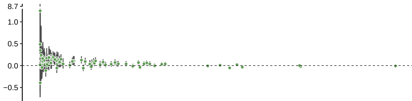
ERA5 data – Extreme low temperature
