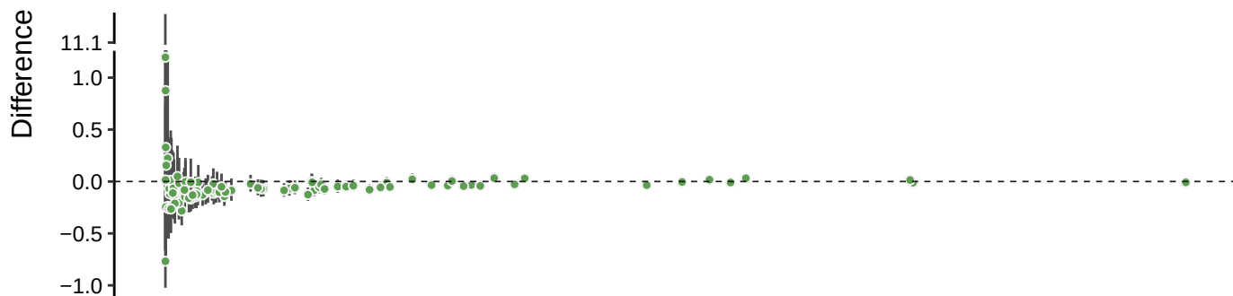
ERA5 data – Extreme high temperature
