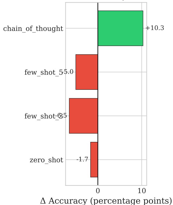
Accuracy
