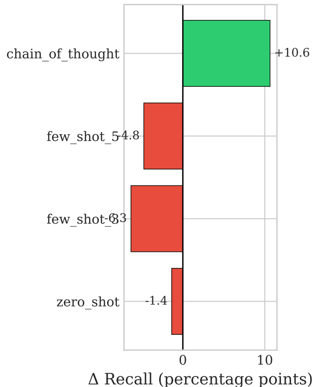
Recall
