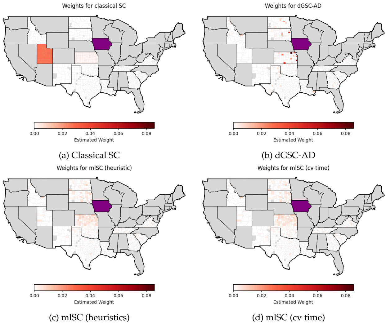
Figure 13: Treated state: Iowa (purple) in 2007 Q2: Weight vectors for control units' counties. Counties with missing data are labeled in grey.
