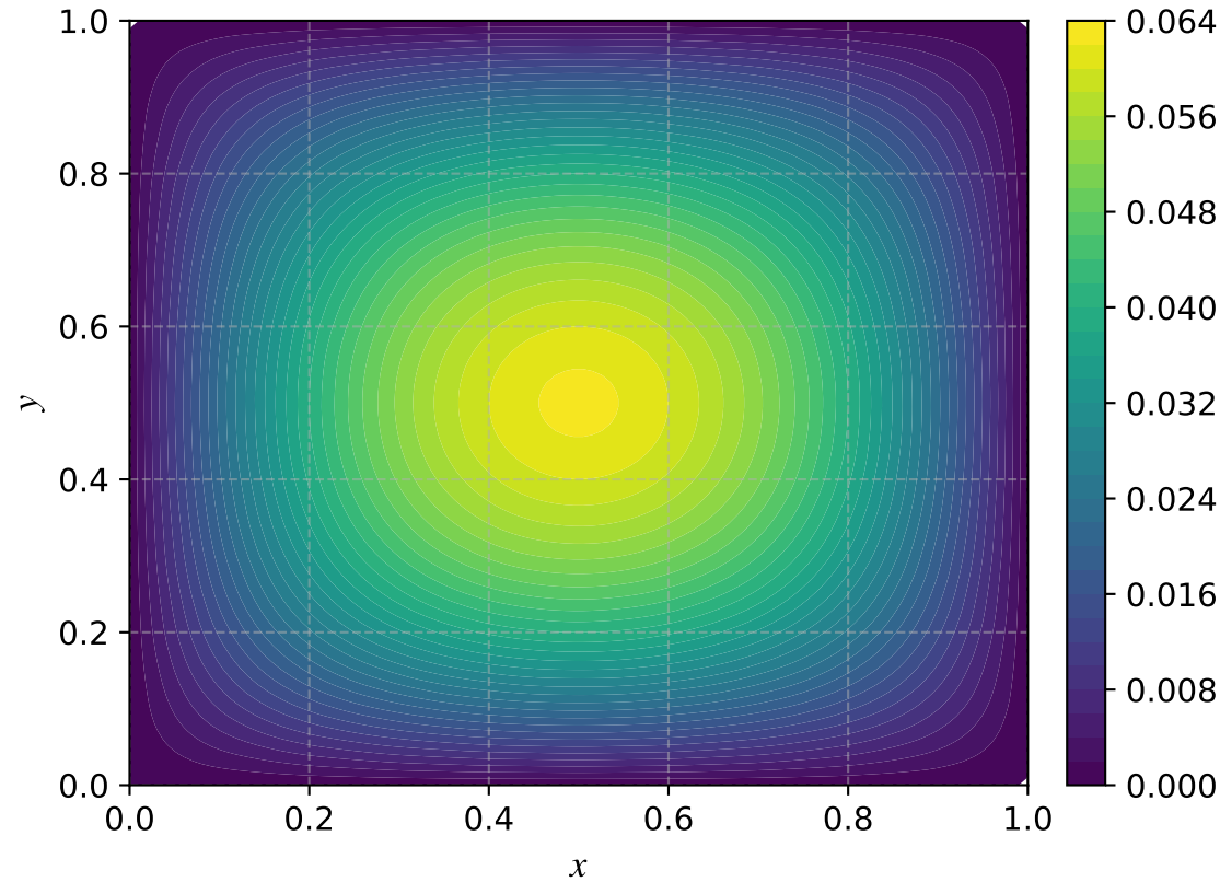
Reduced Solution u_r (Rank r=1 )
