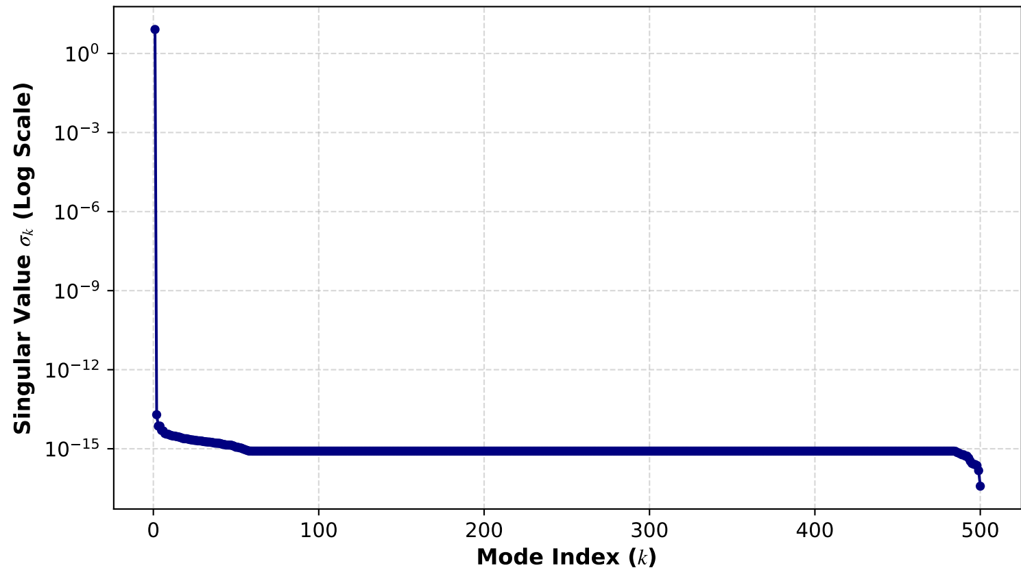
Decay of Singular Values in Snapshot Matrix
