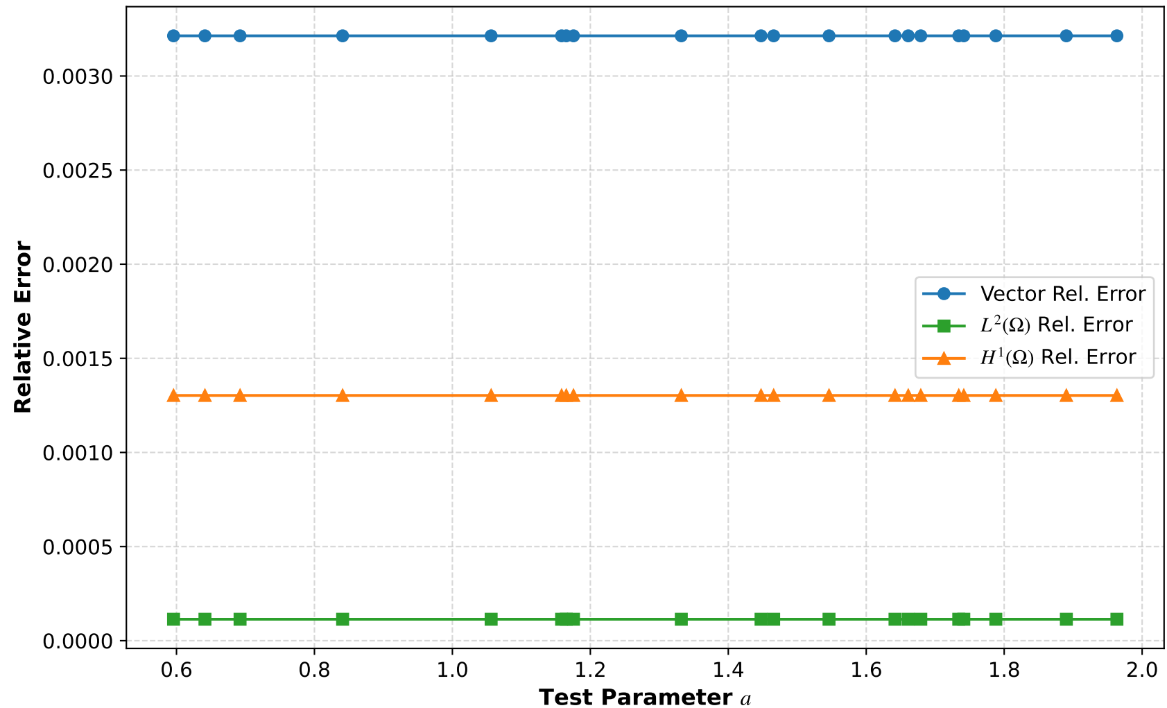
Error of Reduced Order Model against Exact Solution
