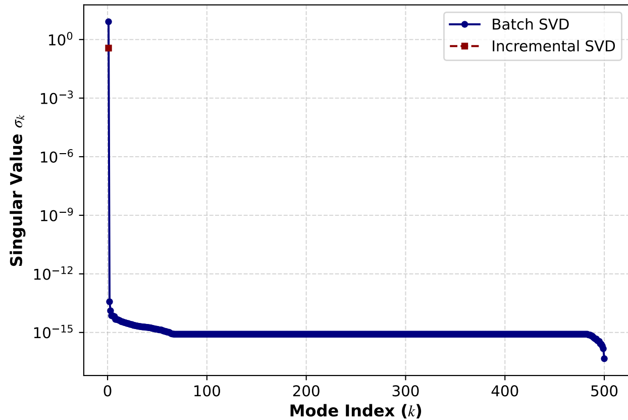
Decay of Singular Values (Batch vs Incremental)
