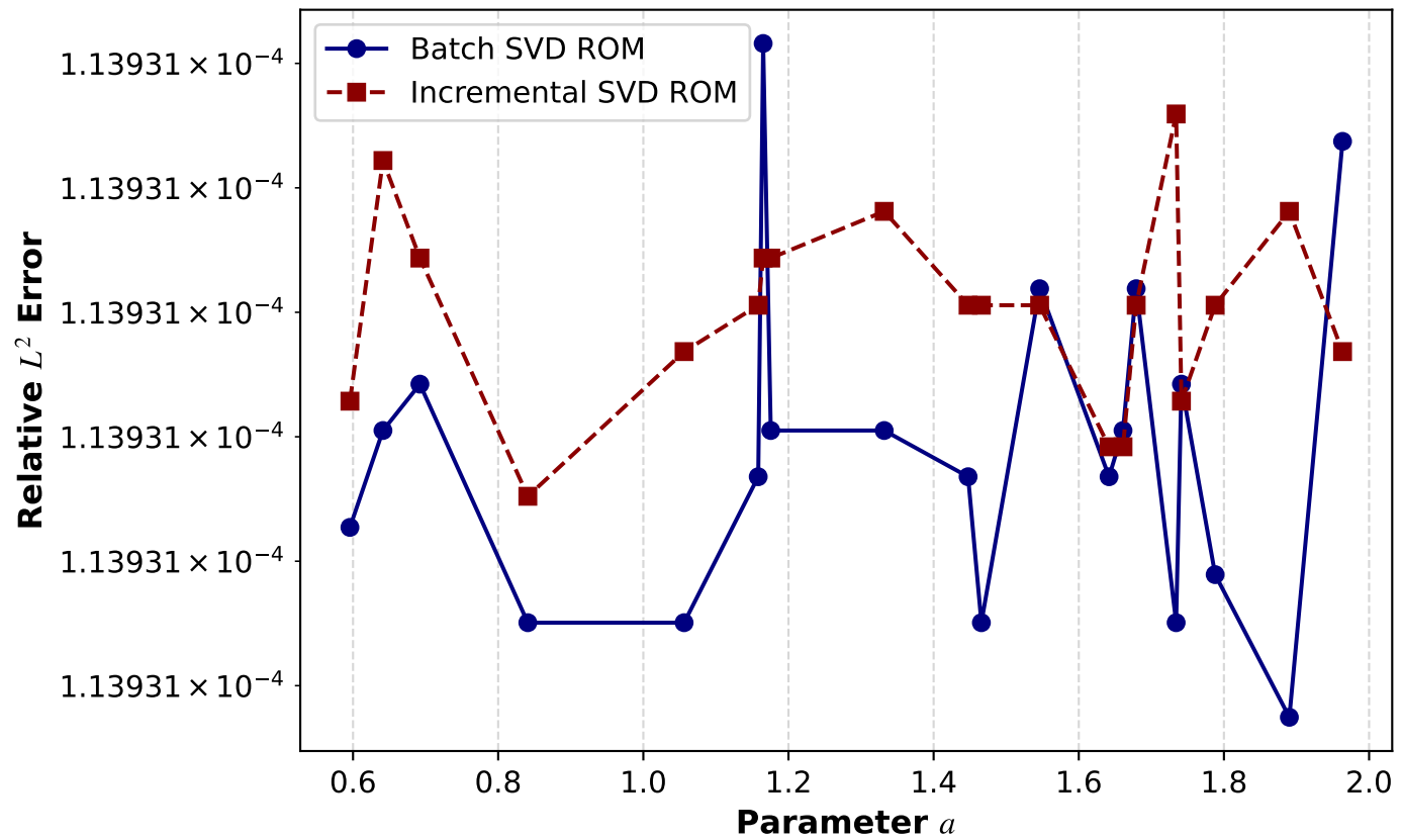
ROM Relative L^2 Error over Test Set
