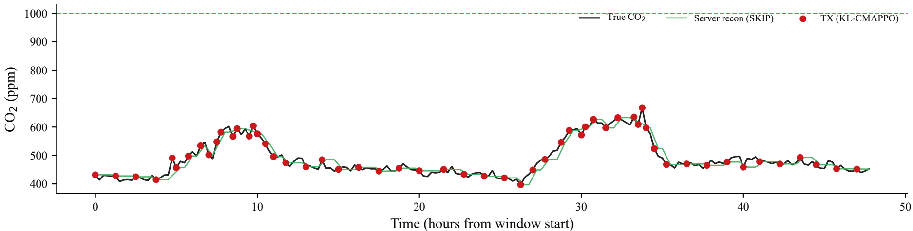
(b) KL-CMAPPO (seed 123, shield OFF) — TX = 56 · reduction vs Fixed-15 = 70.8%
