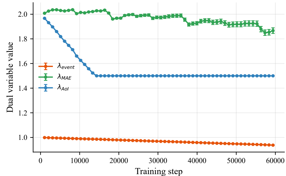
Adaptive Lagrange multipliers
