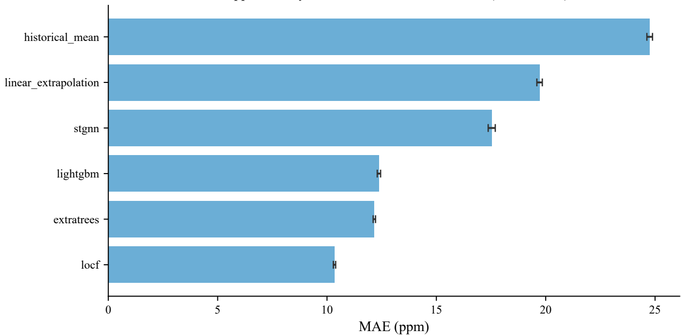
Supplementary: fair reconstruction benchmark (causal mask)
