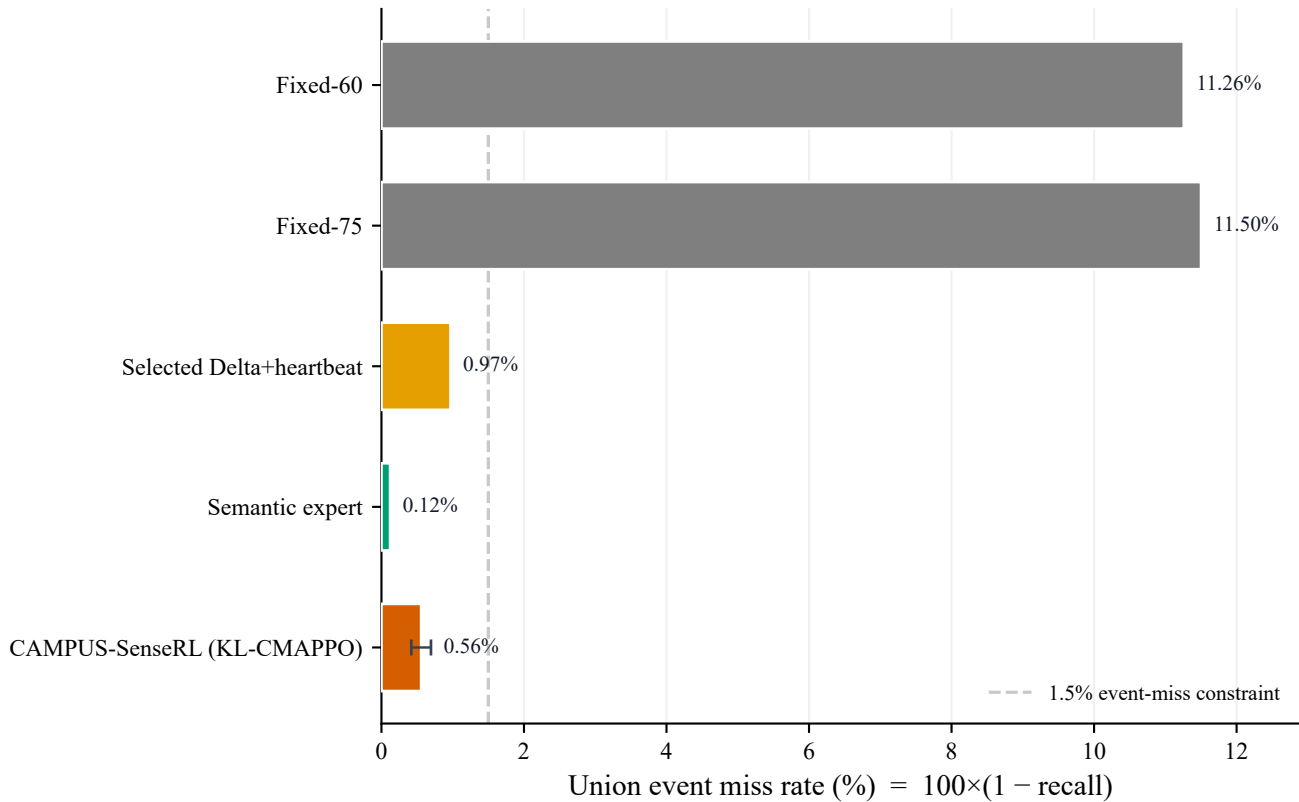
Union-event miss rate on the validation cohort
