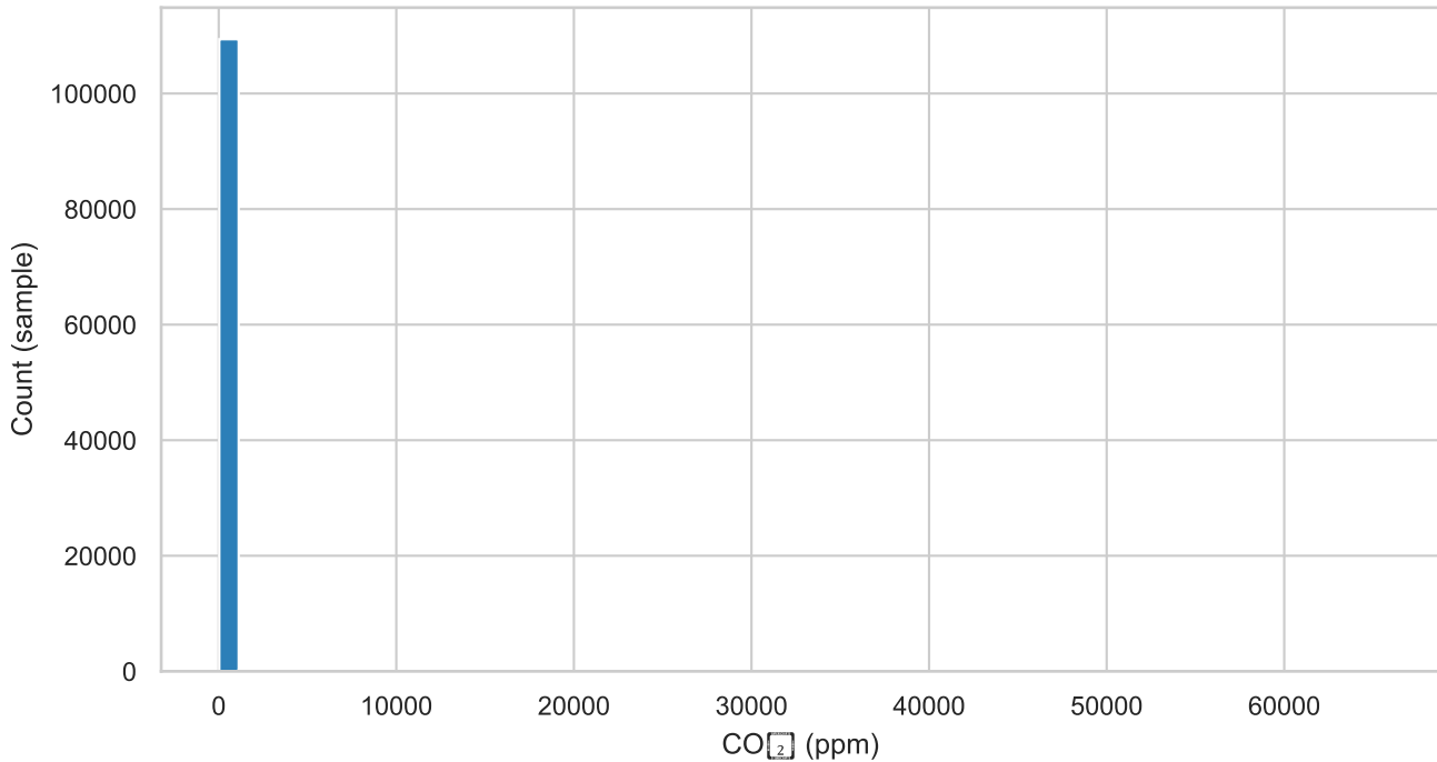
CO 2 distribution (sampled observations)
