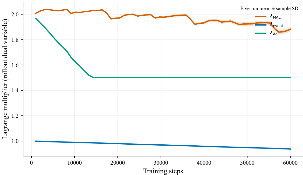
Lagrange multipliers during KL-CMAPPO training (supplementary) Dual variables on rollout estimates — not validation/test feasibility
