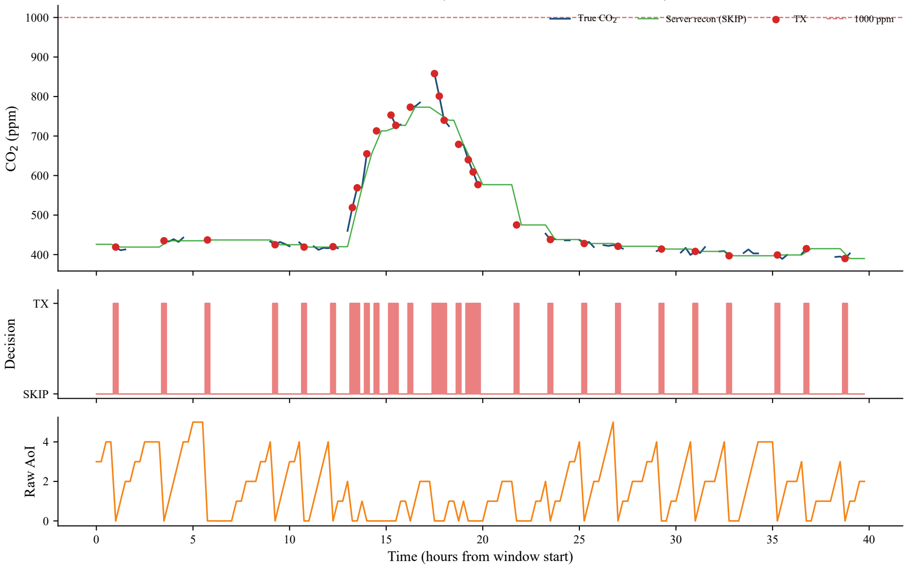
KL-CMAPPO behaviour (seed 123, sensor 030D4E, shield OFF)
