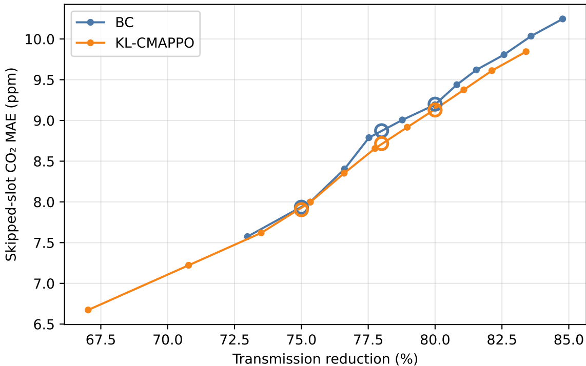
Matched-budget Pareto (validation)
