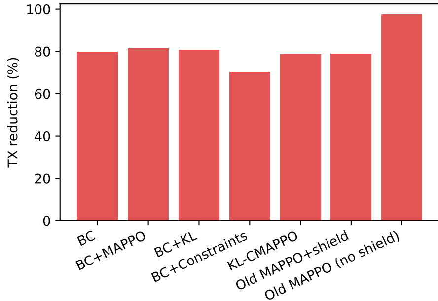
Ablation: communication
