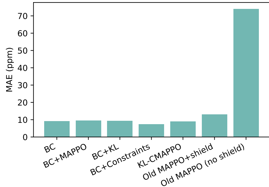
Ablation: reconstruction
