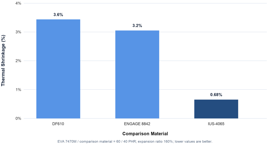
Thermal Shrinkage at 70°C for 40 Minutes
