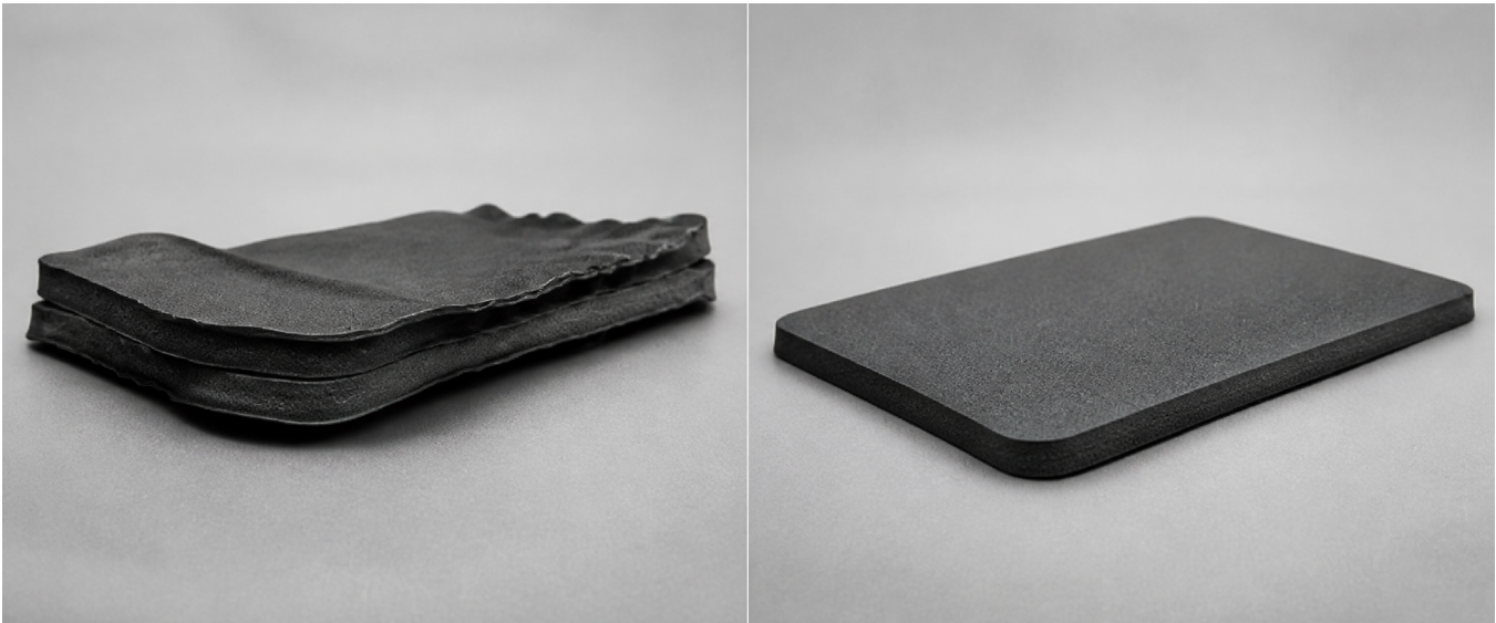
Low-melting material heat deformation versus IUS-4065 dimensional stability
